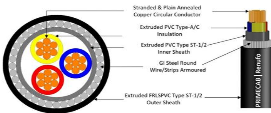
3Core Copper Control Cable as per IS1554-Part1
